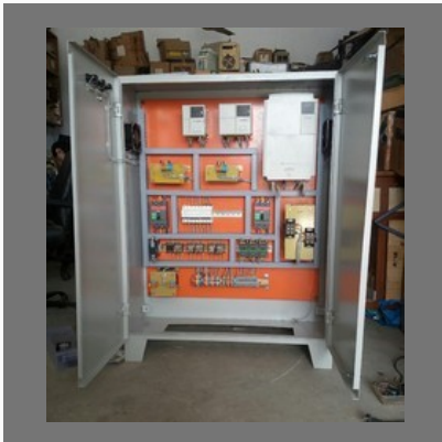
Crene Control Panel (VFD Based)
